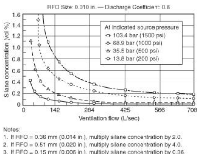
FIGURE 8.5.3(C) Average Silane Concentration in a Ventilated Enclosure.
