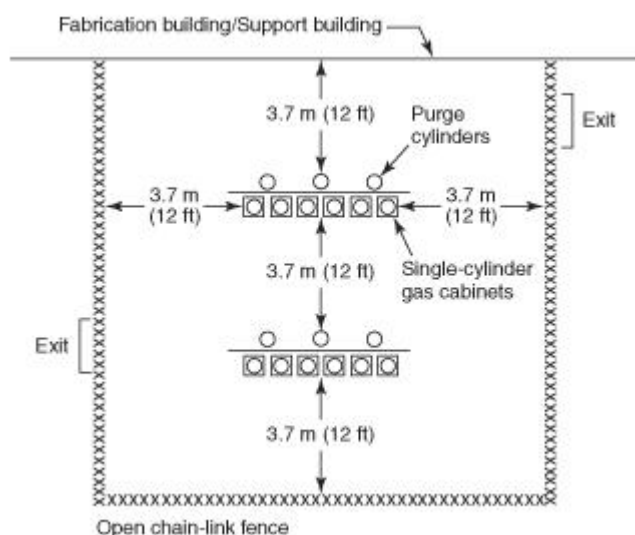
FIGURE 8.5.3 Silane/Toxic Mixes Dispensing Area.
